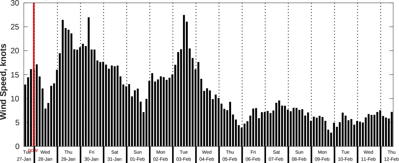
GFS Wind Speed Forecast for NDBC 51209 from 27-Jan-2026 13:00:00 to 12-Feb-2026 13:00:00
