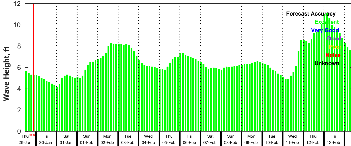
GFS Wave Forecast for NDBC 52211 from 28-Jan-2026 11:00:00 to 13-Feb-2026 11:00:00
