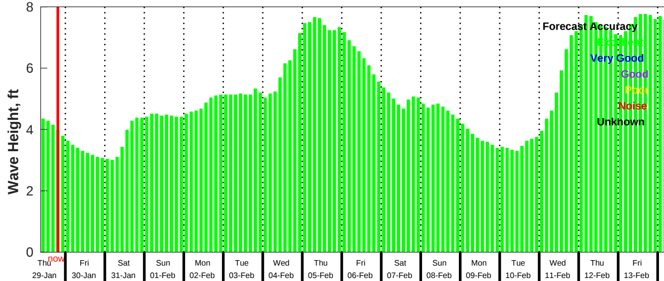
GFS Wave Forecast for NDBC 52212 from 28-Jan-2026 09:00:00 to 13-Feb-2026 09:00:00
