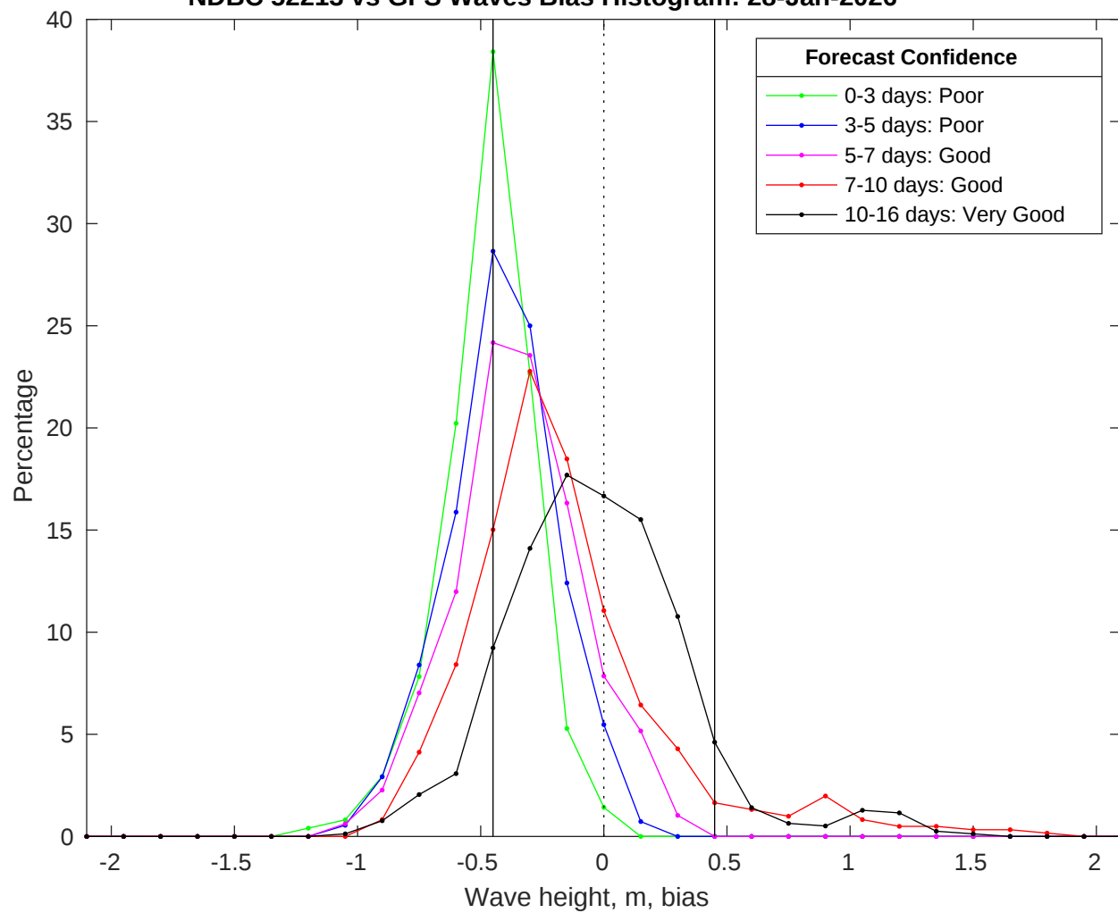
NDBC 52213 vs GFS Waves Bias Histogram: 28-Jan-2026
