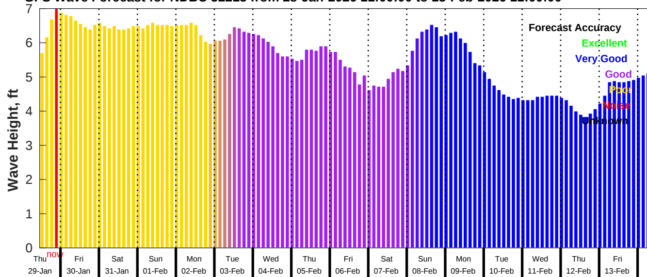
GFS Wave Forecast for NDBC 52213 from 28-Jan-2026 11:00:00 to 13-Feb-2026 11:00:00
