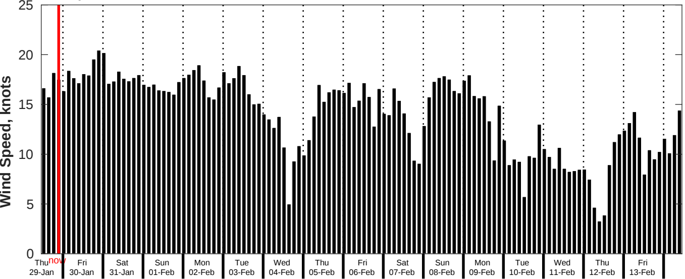
GFS Wind Speed Forecast for NDBC 52213 from 28-Jan-2026 11:00:00 to 13-Feb-2026 11:00:00
