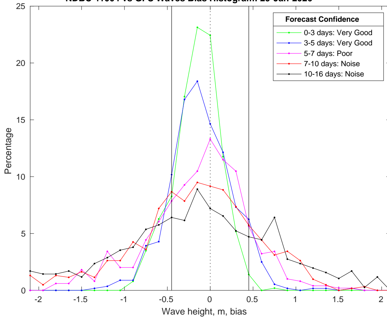
NDBC 41004 vs GFS Waves Bias Histogram: 29-Jan-2026
