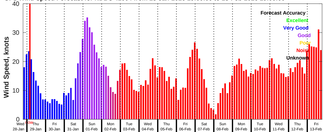
GFS Wind Speed Forecast for NDBC 41004 from 28-Jan-2026 19:00:00 to 13-Feb-2026 19:00:00
