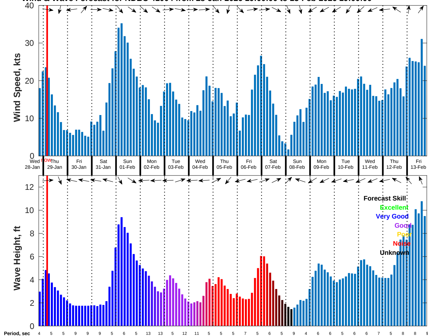
Wind & Wave Forecast for NDBC 41004 from 28-Jan-2026 19:00:00 to 13-Feb-2026 19:00:00
