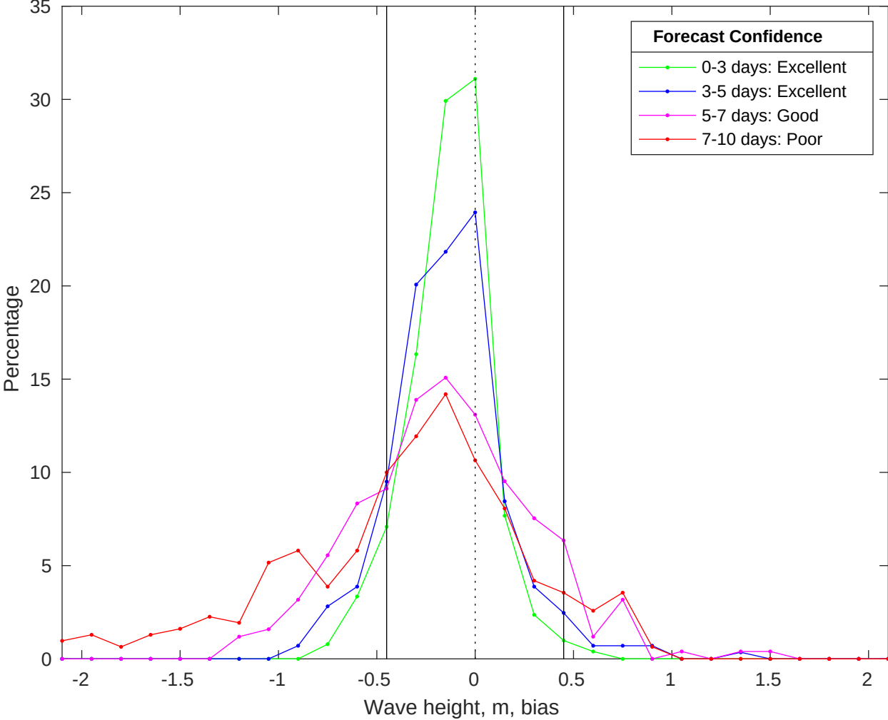
NDBC 41013 vs CMEMS Waves Bias Histogram: 29-Jan-2026
