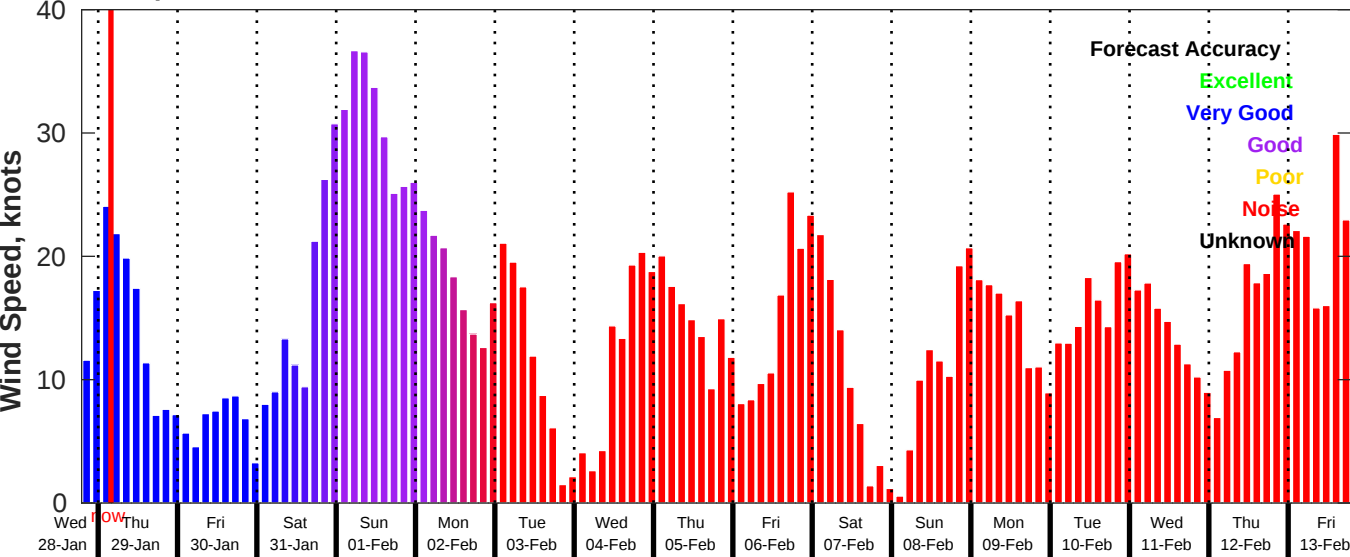
GFS Wind Speed Forecast for NDBC 41013 from 28-Jan-2026 19:00:00 to 13-Feb-2026 19:00:00
