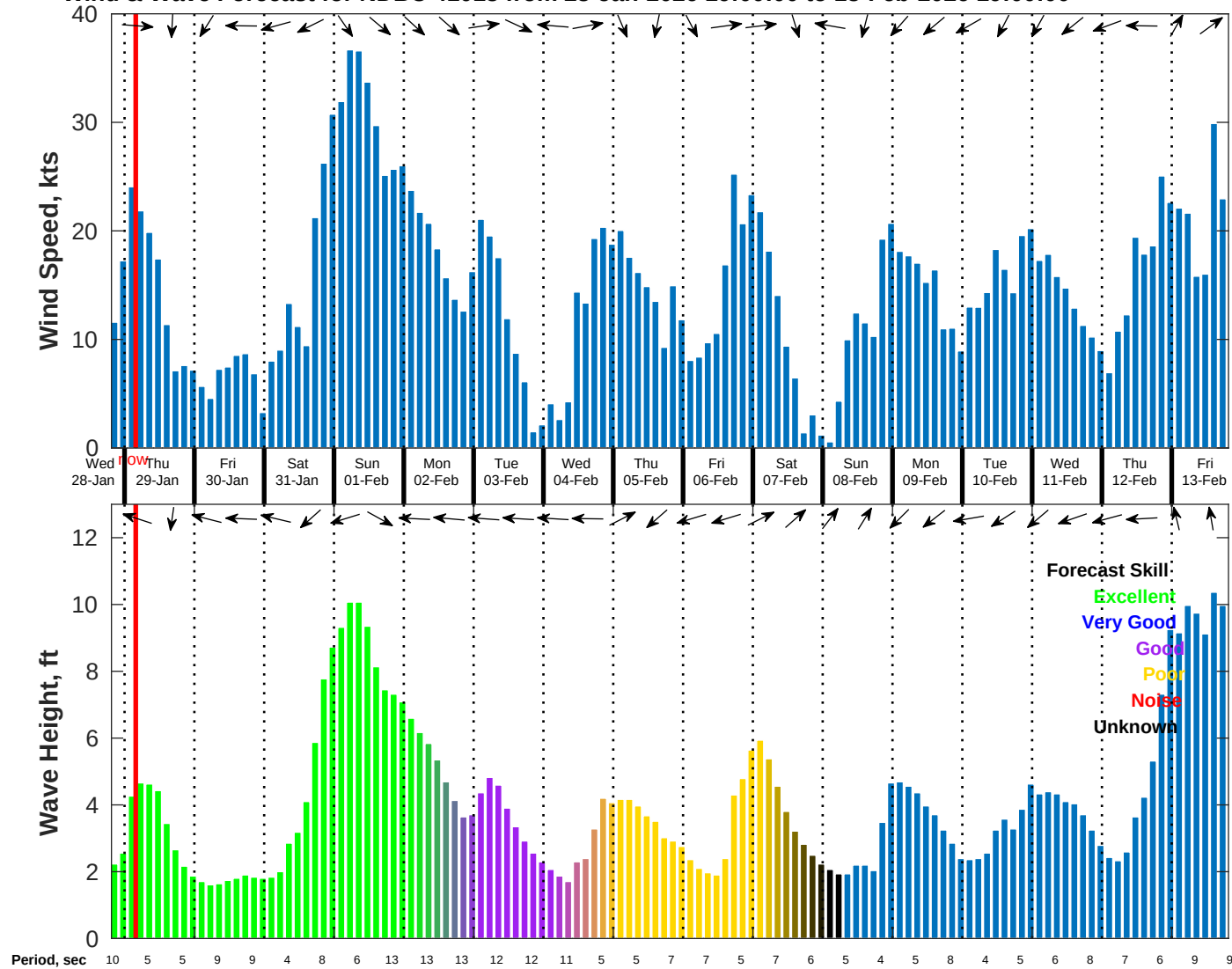
Wind & Wave Forecast for NDBC 41013 from 28-Jan-2026 19:00:00 to 13-Feb-2026 19:00:00
