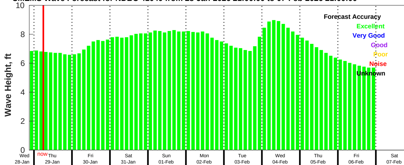
CMEMS Wave Forecast for NDBC 41040 from 28-Jan-2026 21:00:00 to 07-Feb-2026 21:00:00
