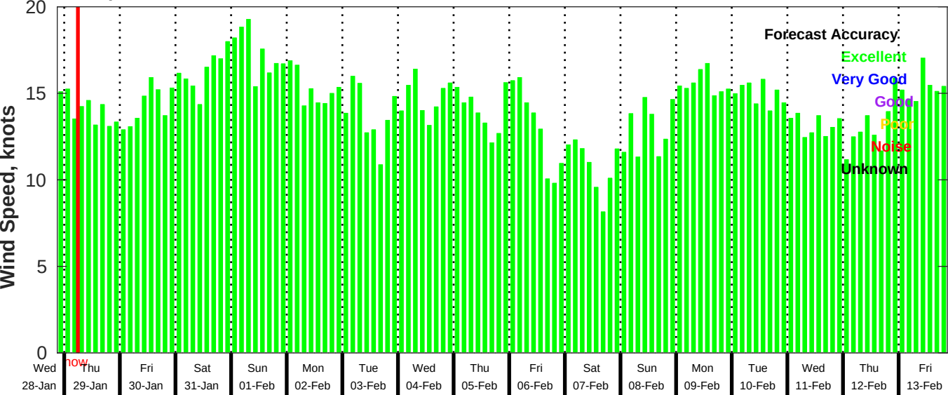
GFS Wind Speed Forecast for NDBC 41040 from 28-Jan-2026 21:00:00 to 13-Feb-2026 21:00:00
