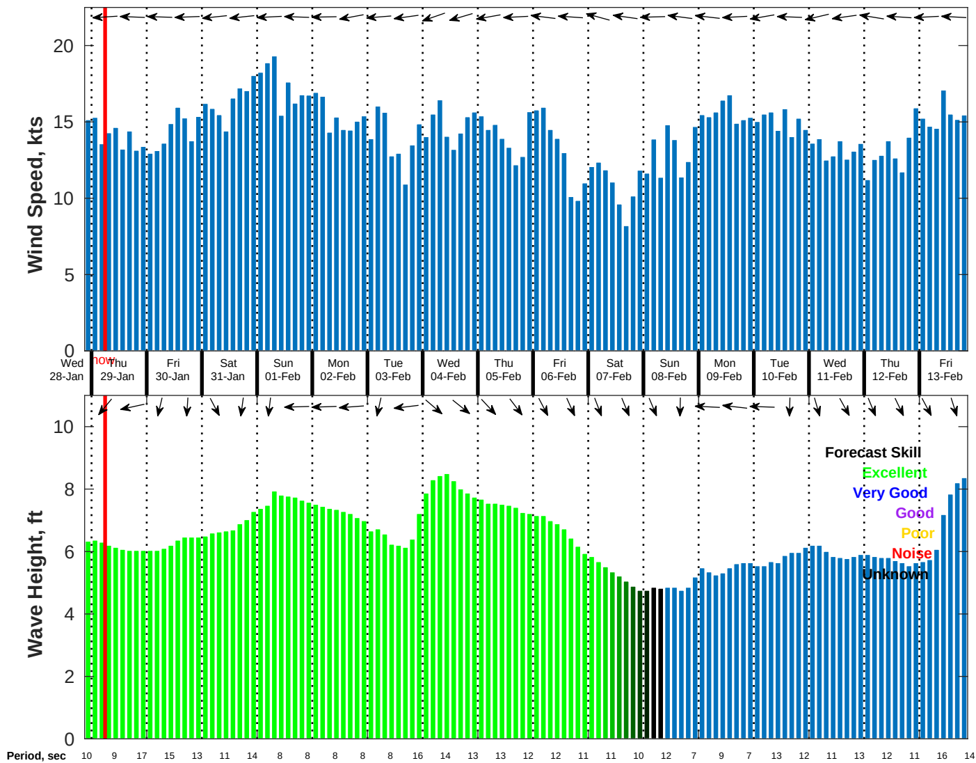
Wind & Wave Forecast for NDBC 41040 from 28-Jan-2026 21:00:00 to 13-Feb-2026 21:00:00
