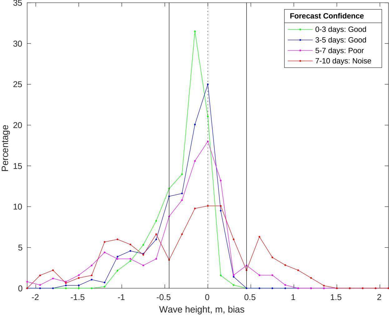
NDBC 42019 vs CMEMS Waves Bias Histogram: 29-Jan-2026
