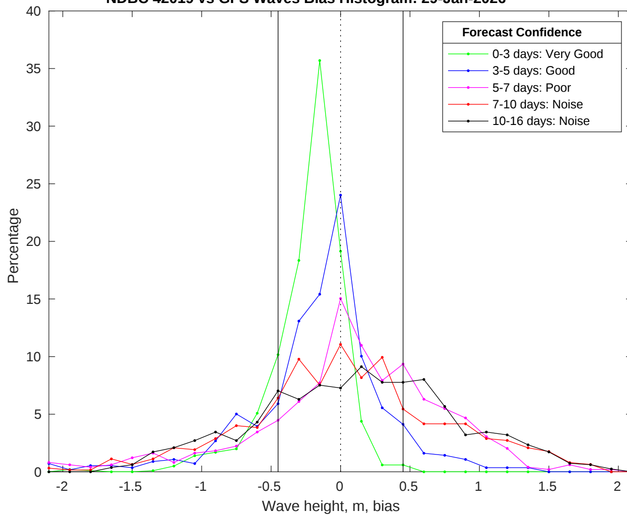
NDBC 42019 vs GFS Waves Bias Histogram: 29-Jan-2026
