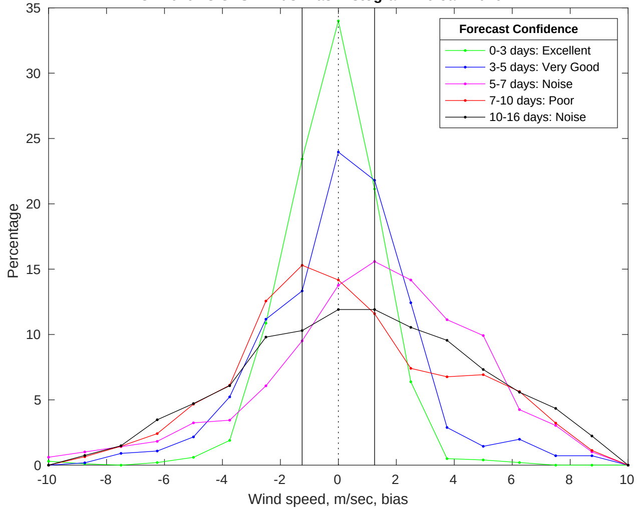
NDBC 42019 vs GFS Winds Bias Histogram: 29-Jan-2026
