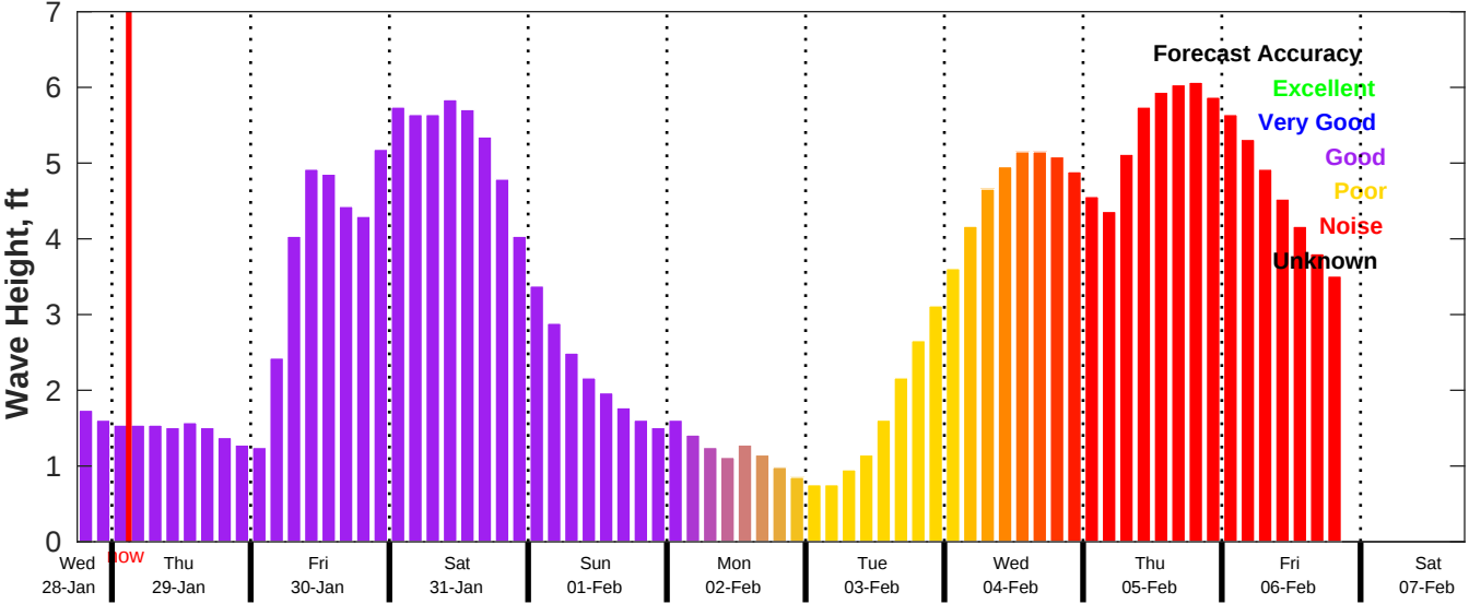
CMEMS Wave Forecast for NDBC 42019 from 28-Jan-2026 18:00:00 to 07-Feb-2026 18:00:00
