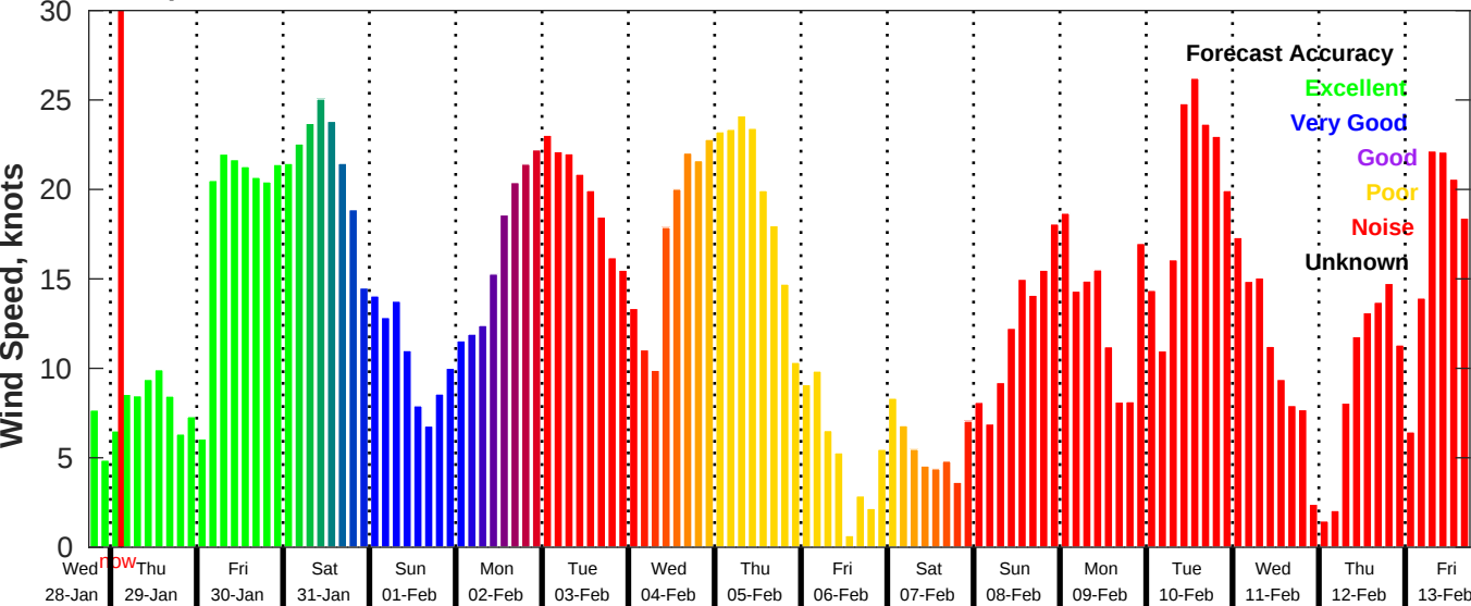
GFS Wind Speed Forecast for NDBC 42019 from 28-Jan-2026 18:00:00 to 13-Feb-2026 18:00:00
