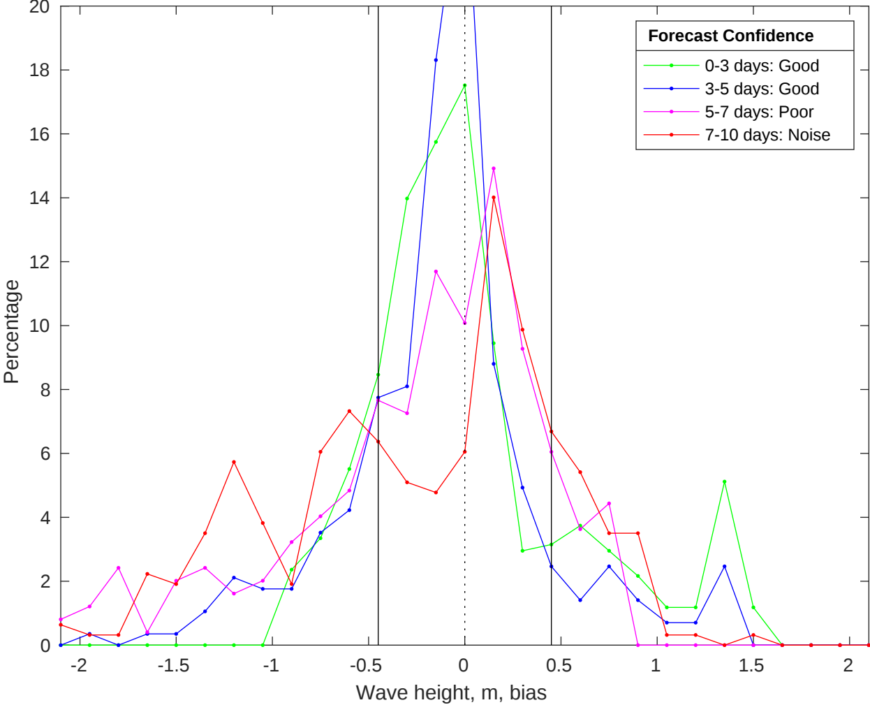
NDBC 42020 vs CMEMS Waves Bias Histogram: 29-Jan-2026
