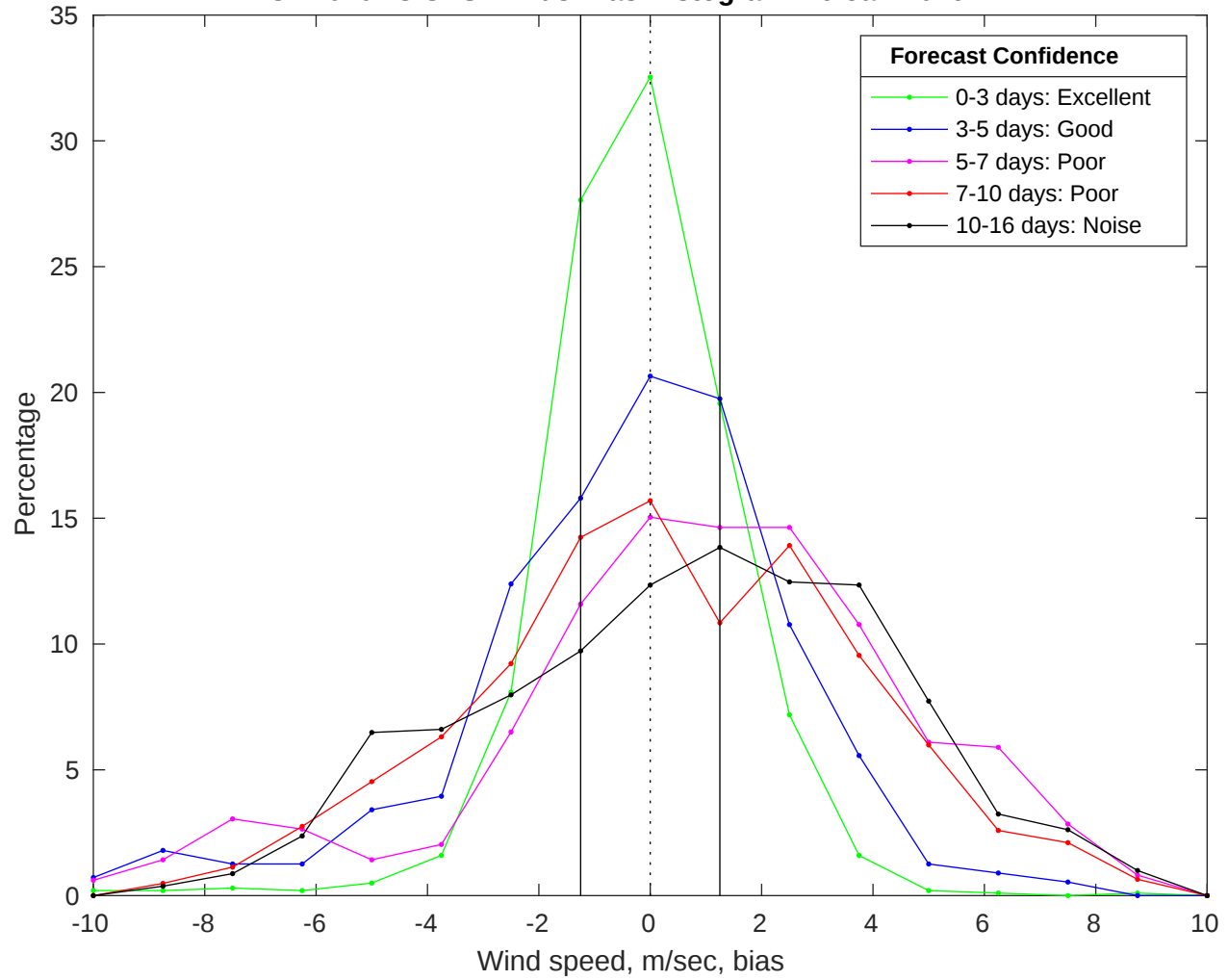
NDBC 42020 vs GFS Winds Bias Histogram: 29-Jan-2026
