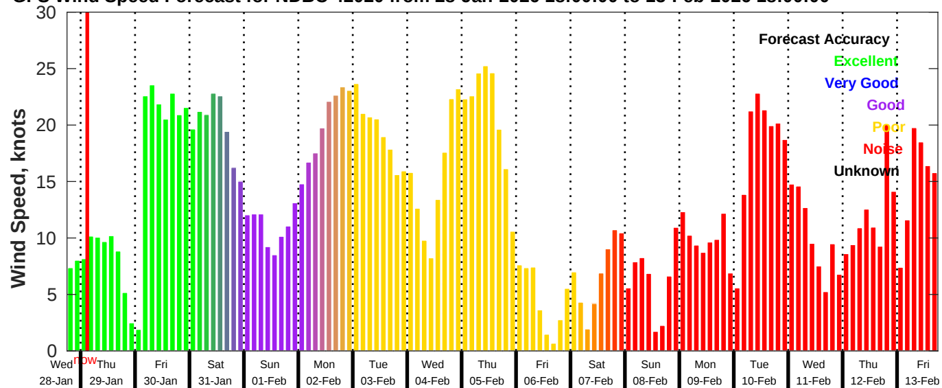
GFS Wind Speed Forecast for NDBC 42020 from 28-Jan-2026 18:00:00 to 13-Feb-2026 18:00:00
