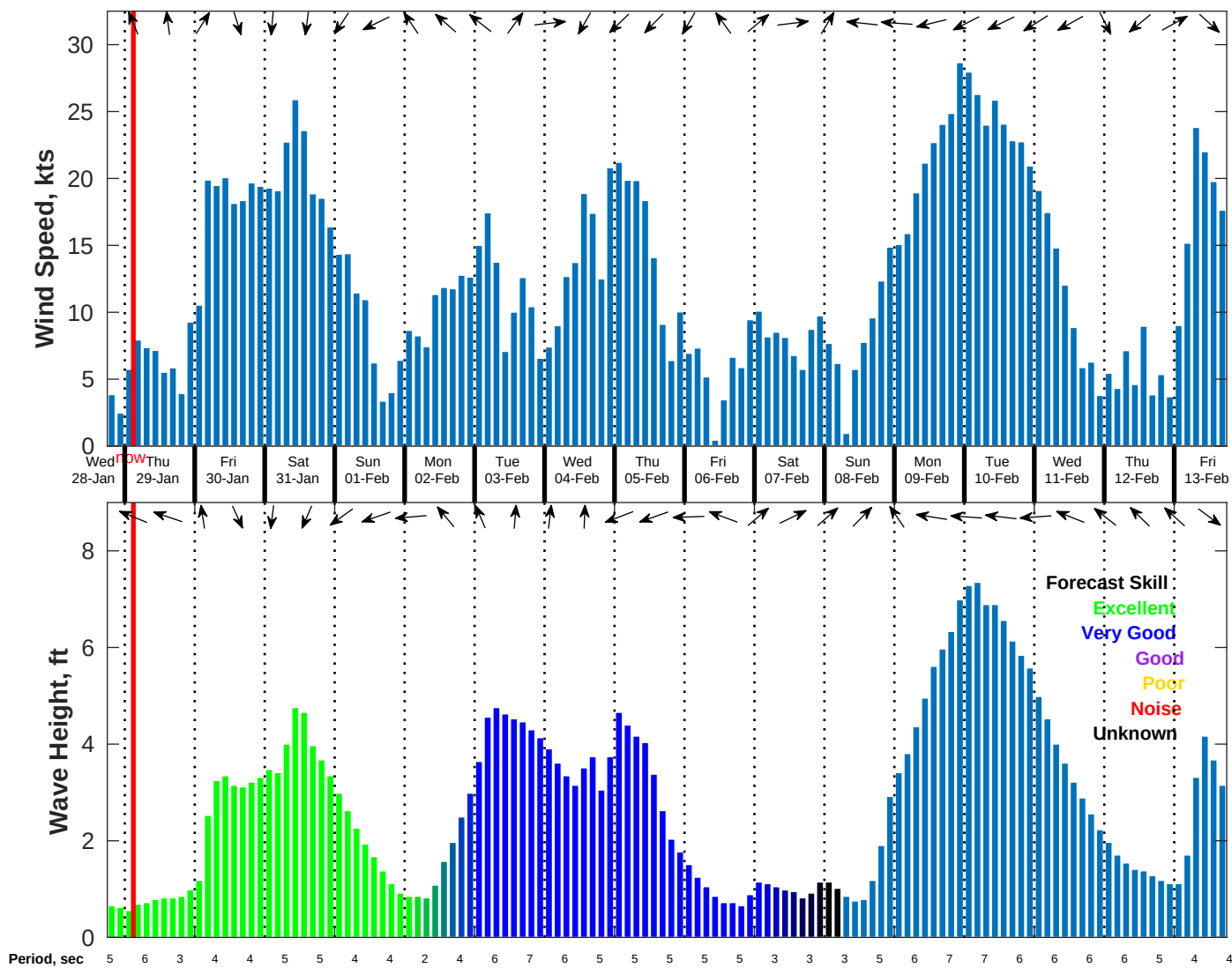
Wind & Wave Forecast for NDBC 42035 from 28-Jan-2026 18:00:00 to 13-Feb-2026 18:00:00
