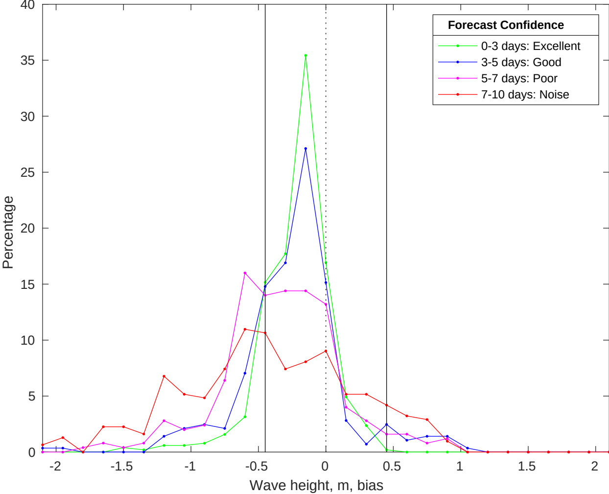
NDBC 42036 vs CMEMS Waves Bias Histogram: 29-Jan-2026
