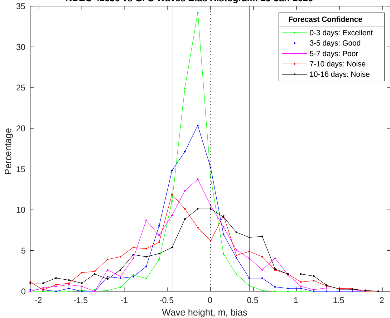
NDBC 42036 vs GFS Waves Bias Histogram: 29-Jan-2026
