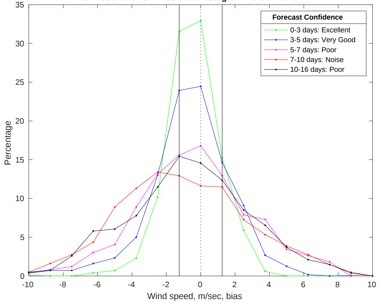
NDBC 42036 vs GFS Winds Bias Histogram: 29-Jan-2026
