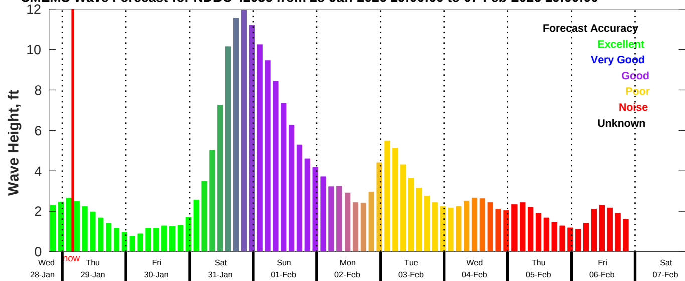
CMEMS Wave Forecast for NDBC 42036 from 28-Jan-2026 19:00:00 to 07-Feb-2026 19:00:00
