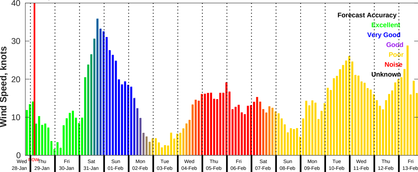
GFS Wind Speed Forecast for NDBC 42036 from 28-Jan-2026 19:00:00 to 13-Feb-2026 19:00:00
