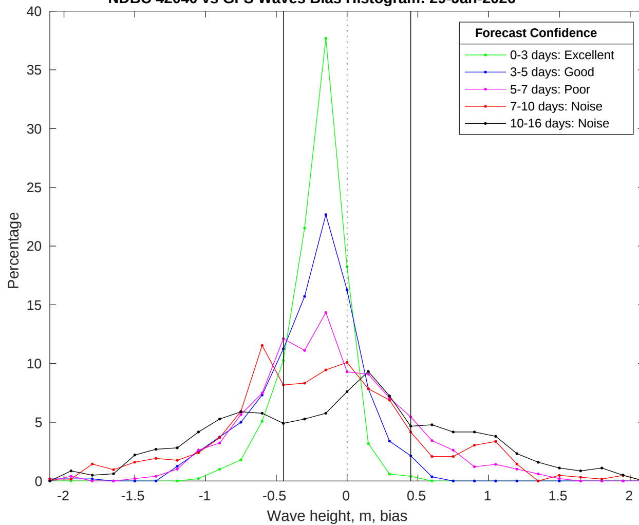
NDBC 42040 vs GFS Waves Bias Histogram: 29-Jan-2026
