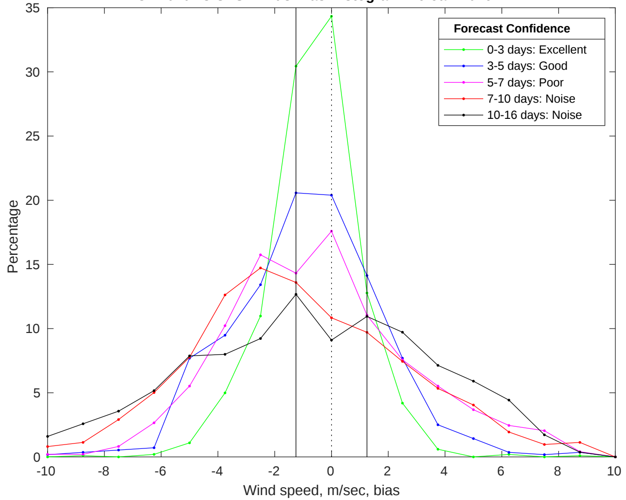
NDBC 42040 vs GFS Winds Bias Histogram: 29-Jan-2026
