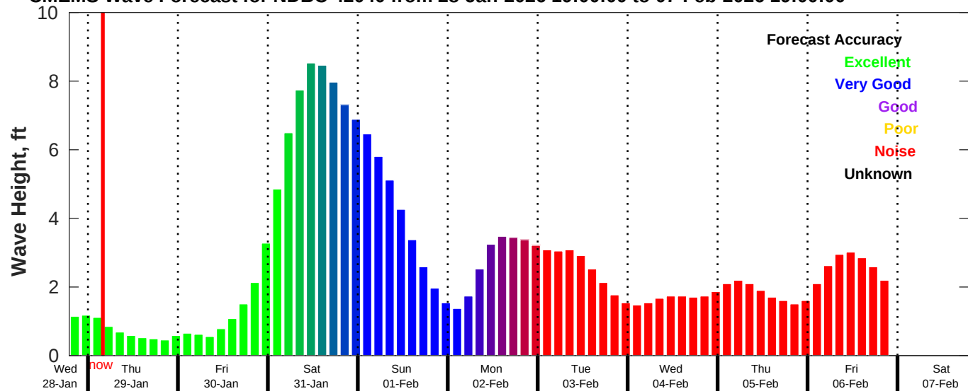
CMEMS Wave Forecast for NDBC 42040 from 28-Jan-2026 19:00:00 to 07-Feb-2026 19:00:00
