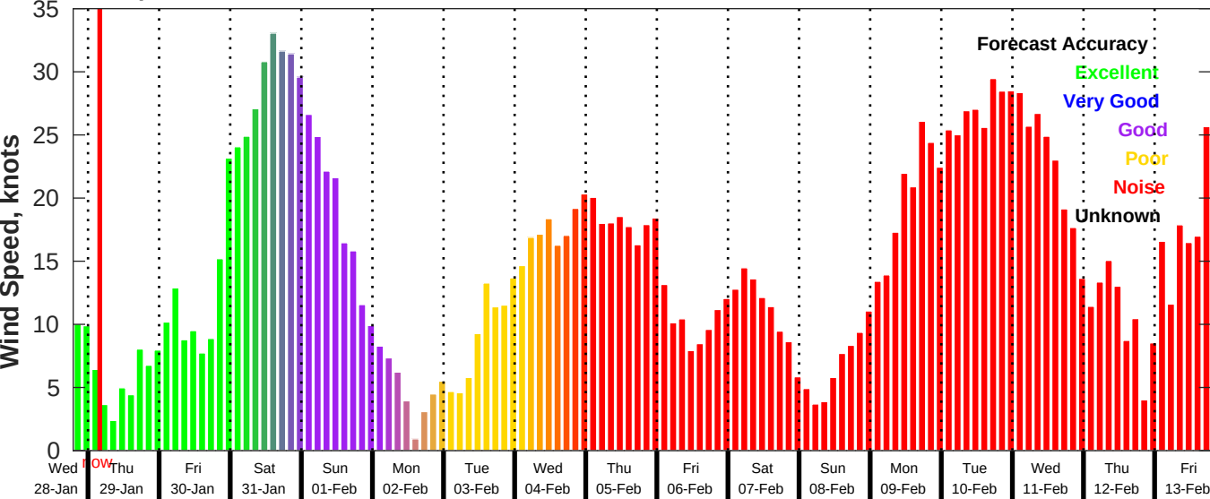
GFS Wind Speed Forecast for NDBC 42040 from 28-Jan-2026 19:00:00 to 13-Feb-2026 19:00:00
