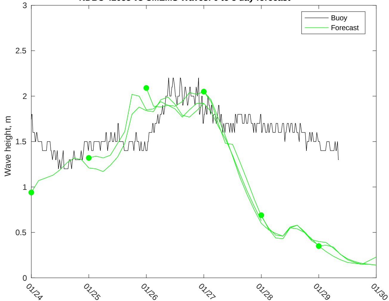
NDBC 42058 vs CMEMS Waves: 0 to 3 day forecast
