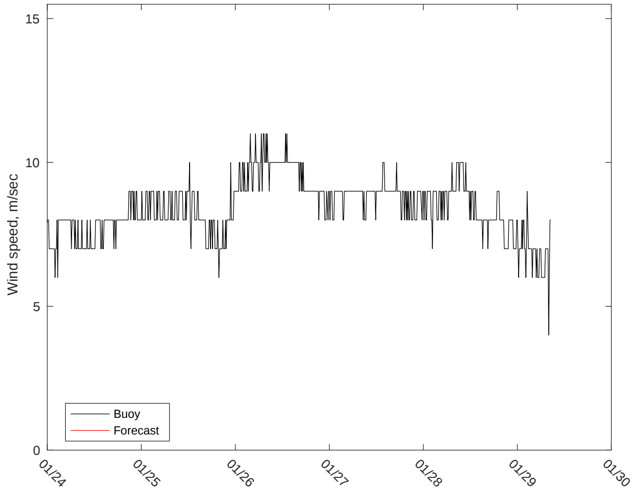
NDBC 42058 vs GFS Winds: 10 to 16 day forecast
