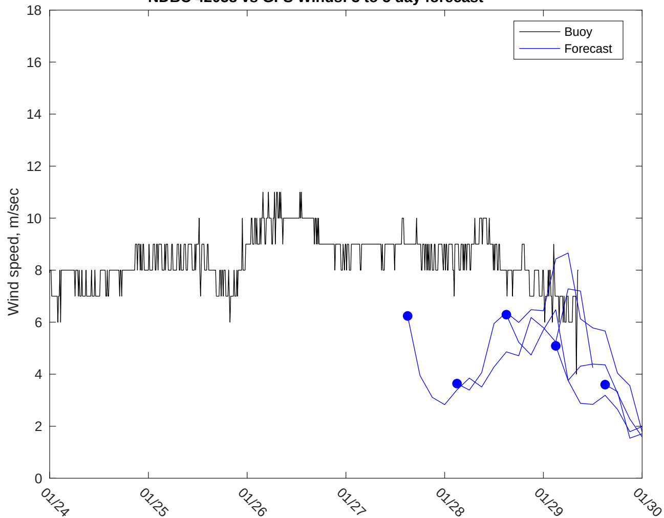
NDBC 42058 vs GFS Winds: 3 to 5 day forecast
