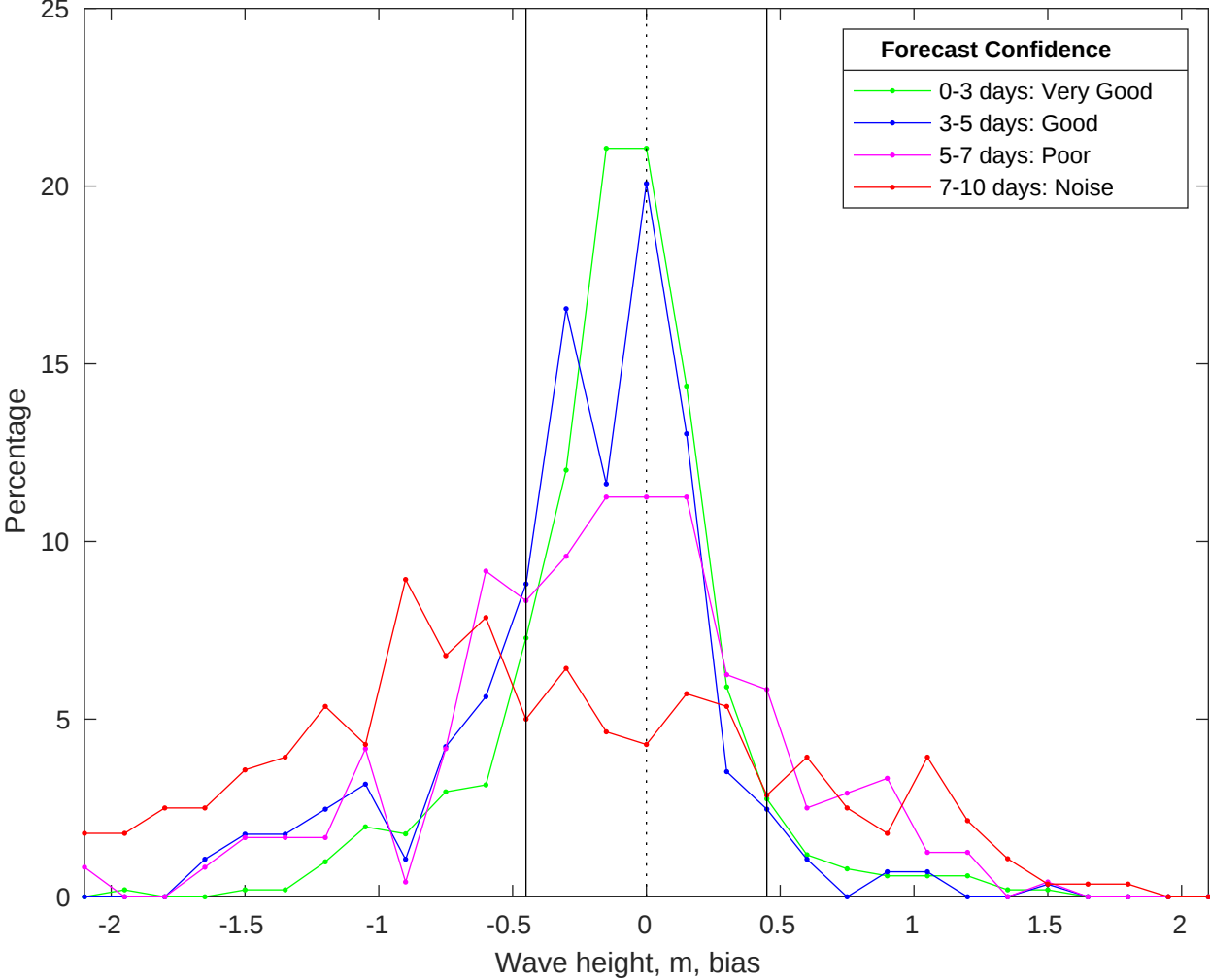
NDBC 44008 vs CMEMS Waves Bias Histogram: 29-Jan-2026
