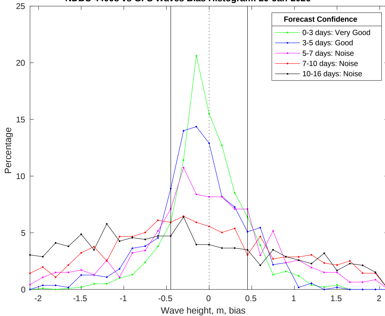
NDBC 44008 vs GFS Waves Bias Histogram: 29-Jan-2026
