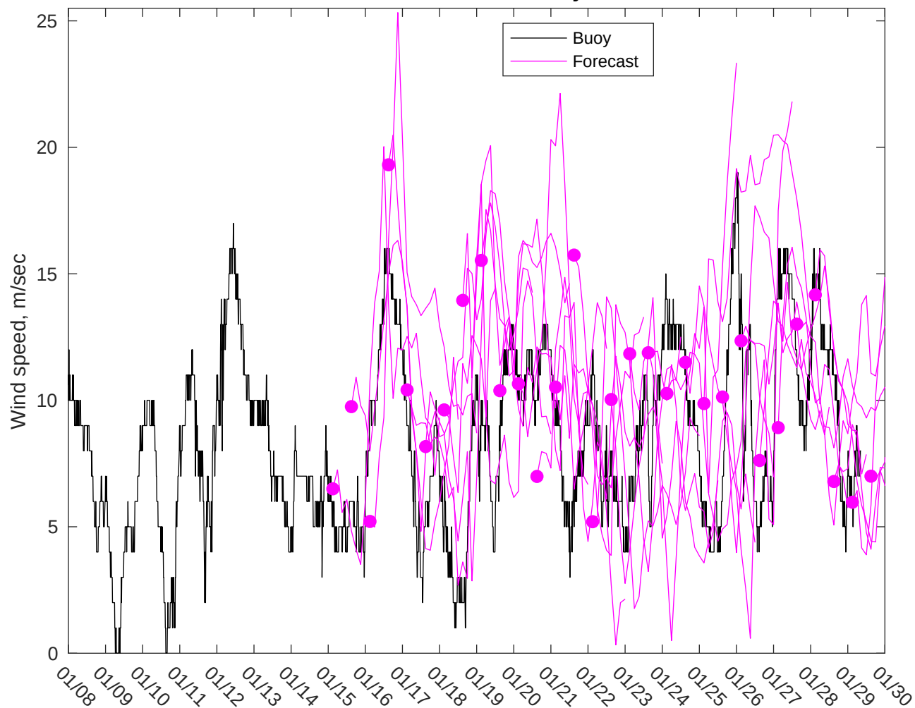
NDBC 44008 vs GFS Winds: 7 to 10 day forecast
