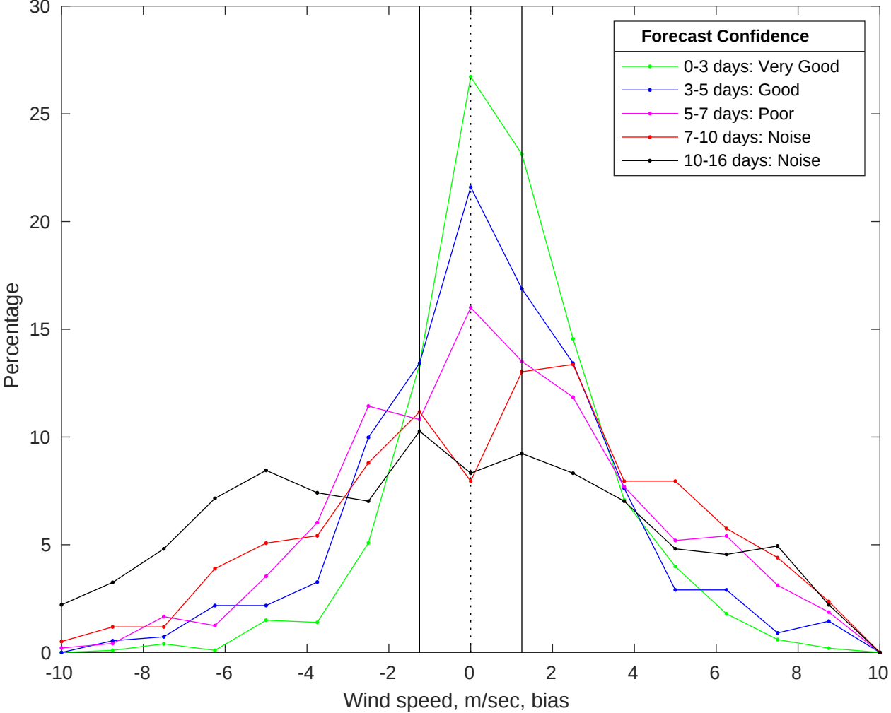
NDBC 44008 vs GFS Winds Bias Histogram: 29-Jan-2026
