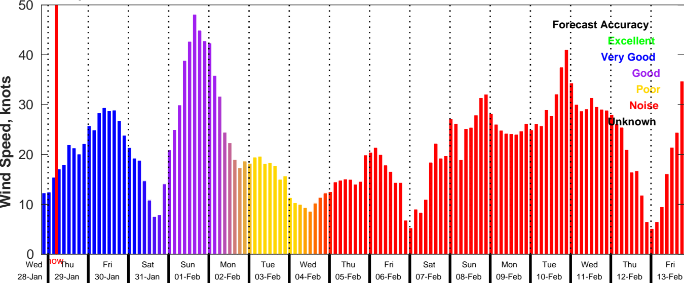
GFS Wind Speed Forecast for NDBC 44008 from 28-Jan-2026 20:00:00 to 13-Feb-2026 20:00:00
