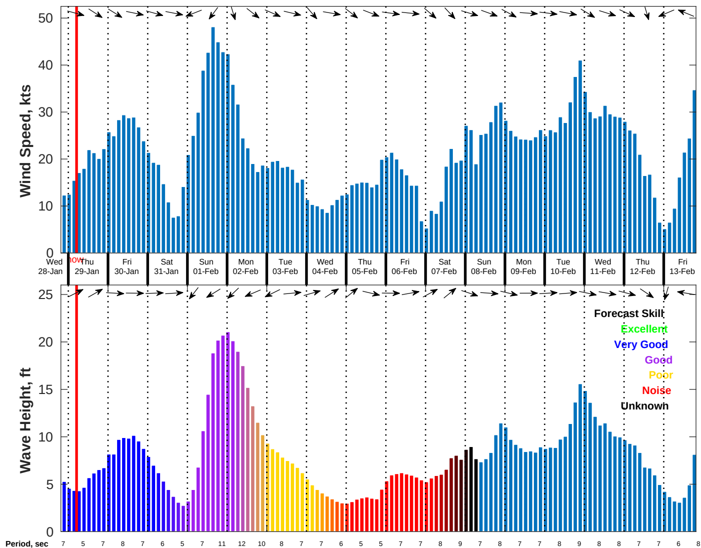
Wind & Wave Forecast for NDBC 44008 from 28-Jan-2026 20:00:00 to 13-Feb-2026 20:00:00
