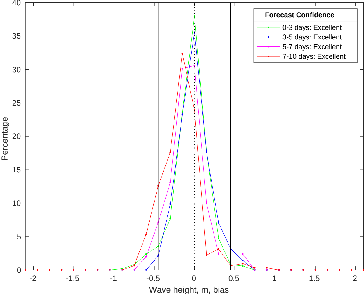
NDBC 46011 vs CMEMS Waves Bias Histogram: 29-Jan-2026
