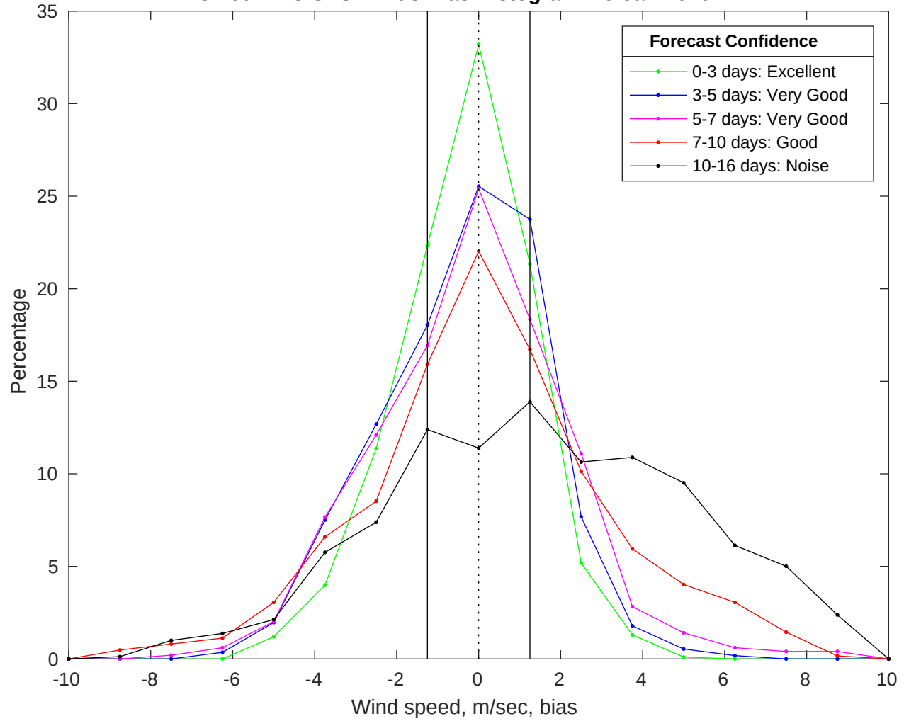
NDBC 46011 vs GFS Winds Bias Histogram: 29-Jan-2026
