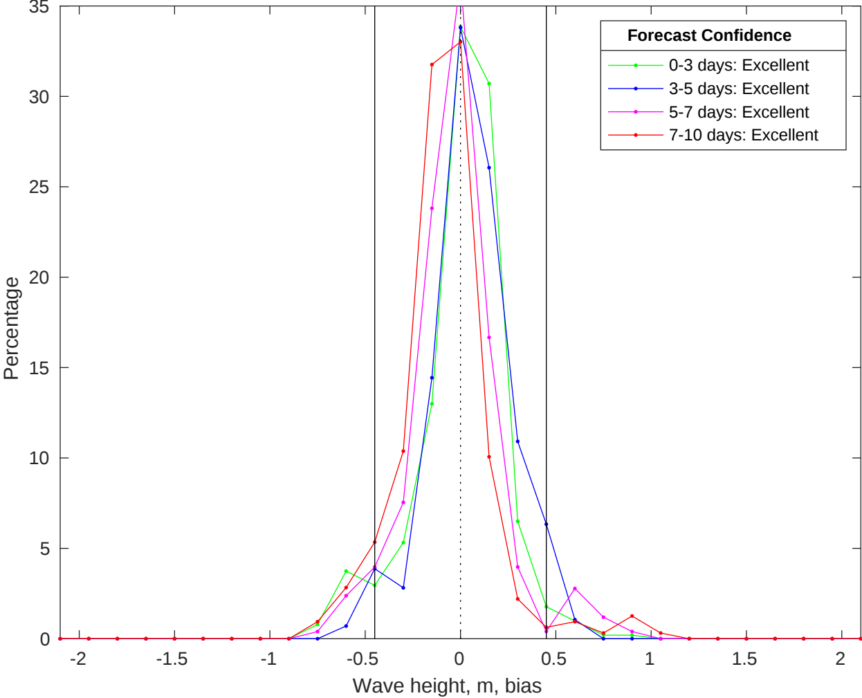
NDBC 46028 vs CMEMS Waves Bias Histogram: 29-Jan-2026
