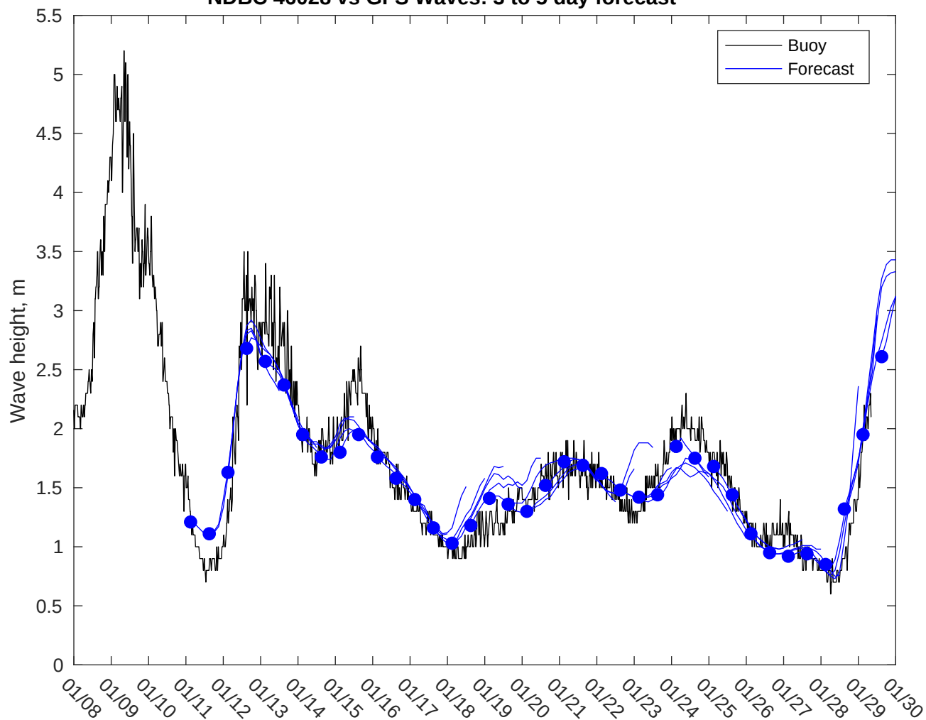
NDBC 46028 vs GFS Waves: 3 to 5 day forecast
