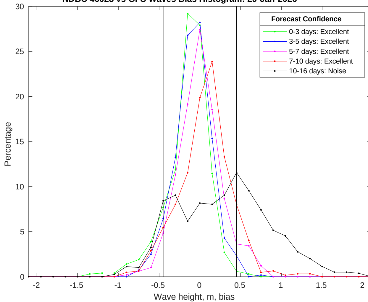
NDBC 46028 vs GFS Waves Bias Histogram: 29-Jan-2026
