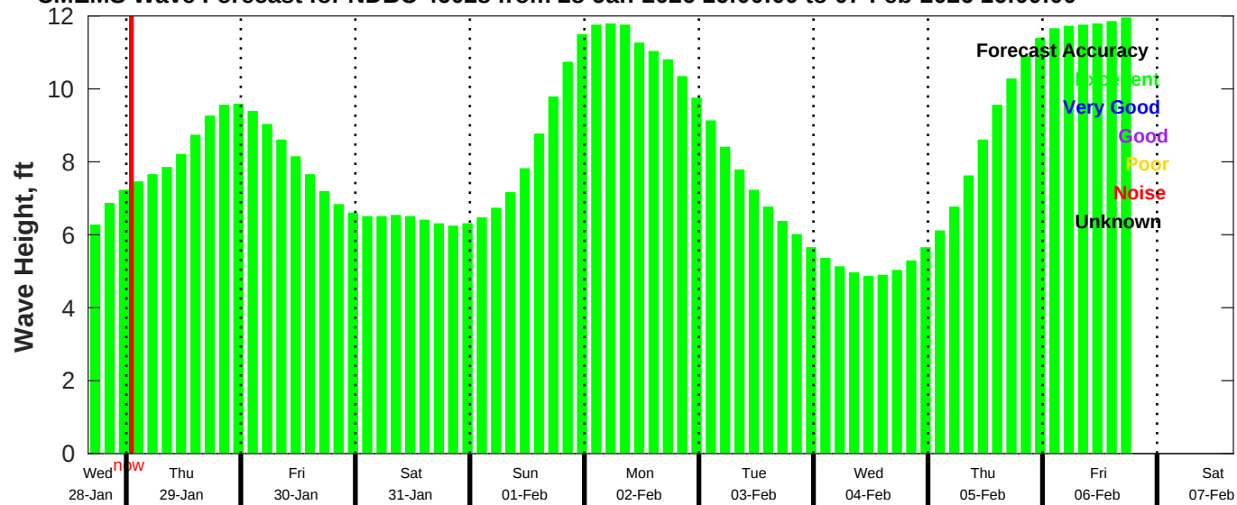
CMEMS Wave Forecast for NDBC 46028 from 28-Jan-2026 16:00:00 to 07-Feb-2026 16:00:00
