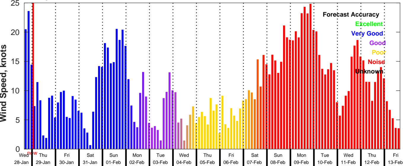
GFS Wind Speed Forecast for NDBC 46054 from 28-Jan-2026 16:00:00 to 13-Feb-2026 16:00:00
