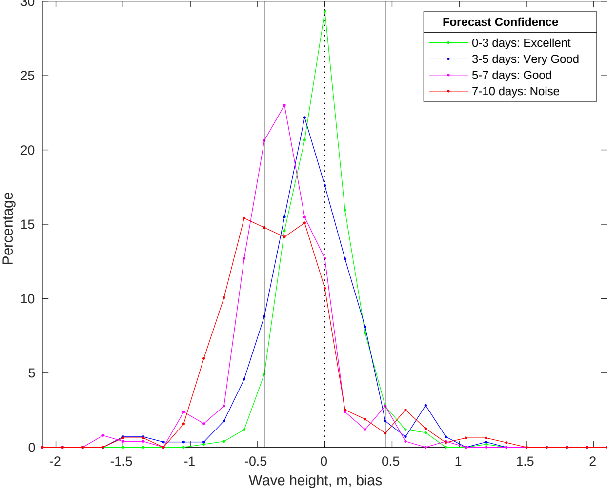
NDBC 46059 vs CMEMS Waves Bias Histogram: 29-Jan-2026
